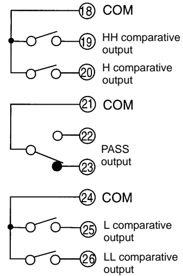
K3NX with 5 Relay Output Boards, K31-C5
