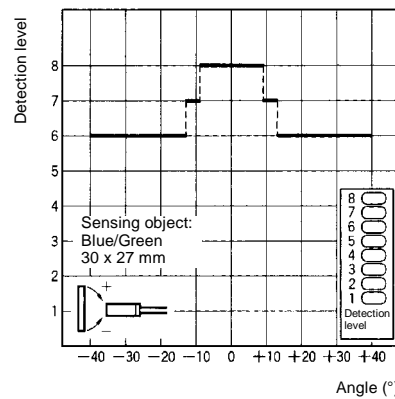
E3MC-(M)Xj j (X Direction)
