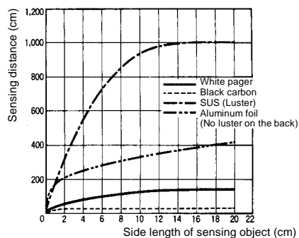
Size of Sensing Object vs. Sensing Distance E3JM-DS70j 4(T)
