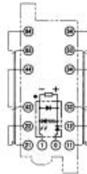
G7SA-4A2B Mounted
