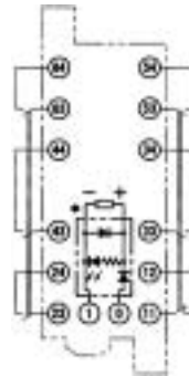
G7SA-5A1B Mounted
