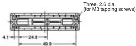
G7SA-3A3B Mounted
